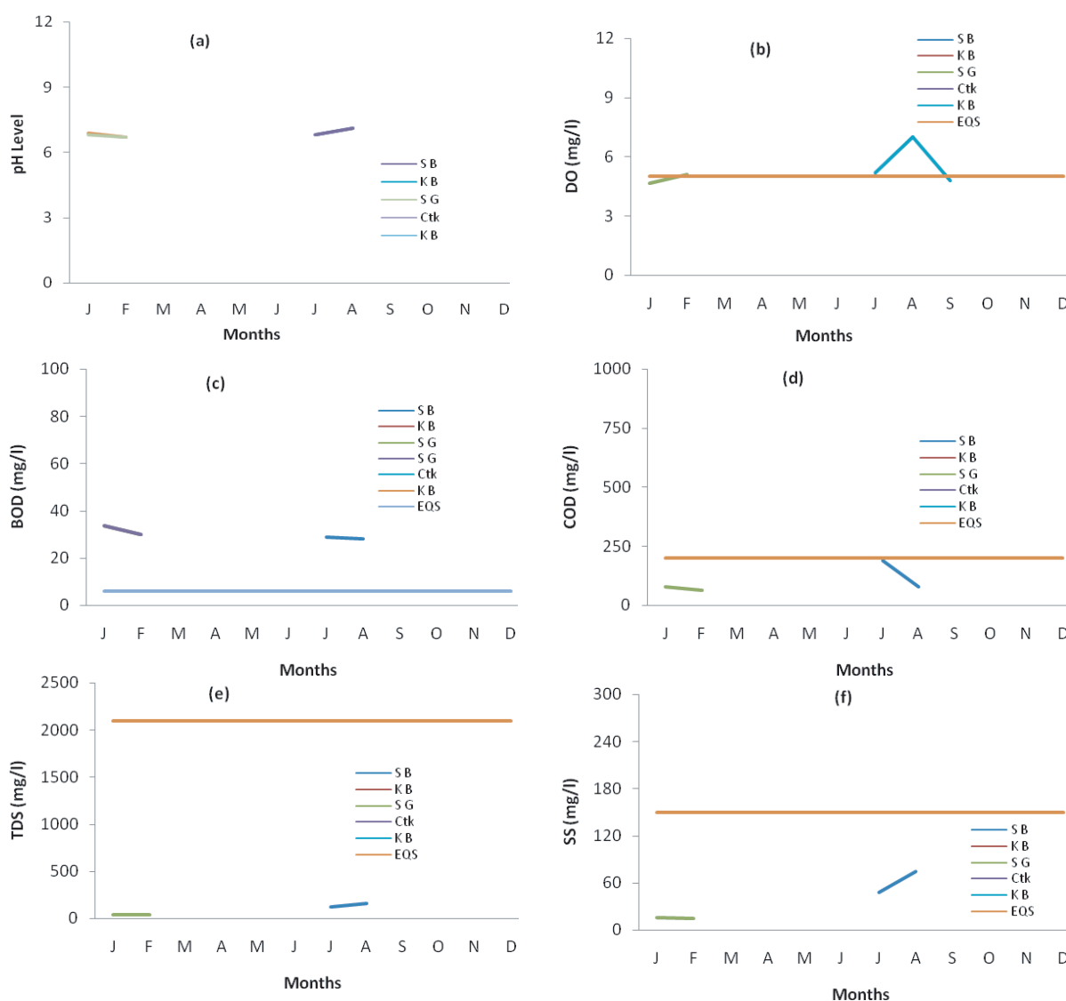
Fig.23. Graphical presentation of pH, DO, BOD, TDS, COD and SS of Surma river in 2014
